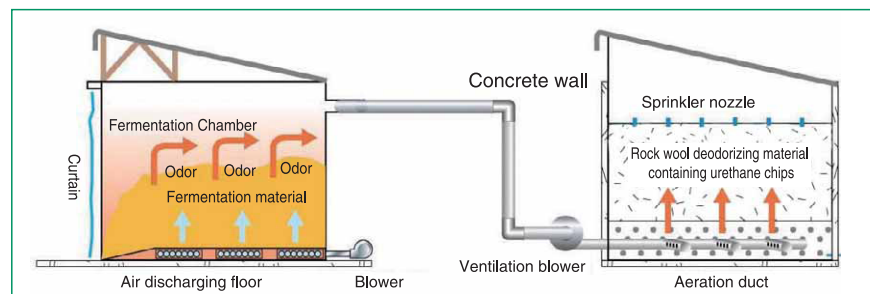
Rock wool deodorization system mechanism
