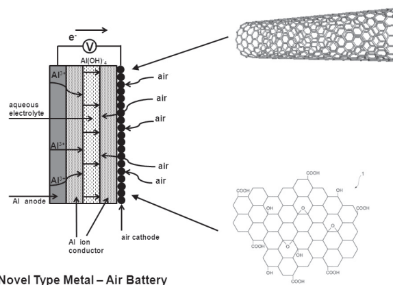
Novel Type Metal - Air Battery
